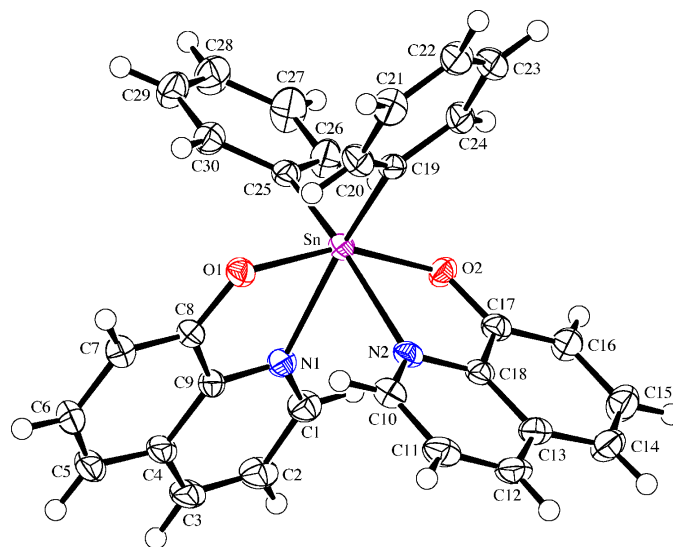
Figure 1 A view of the molecule of (I), showing the atom-labelling scheme. Displacement ellipsoids are drawn at the 50% probability level and H atoms are represented by spheres of arbitrary size.
